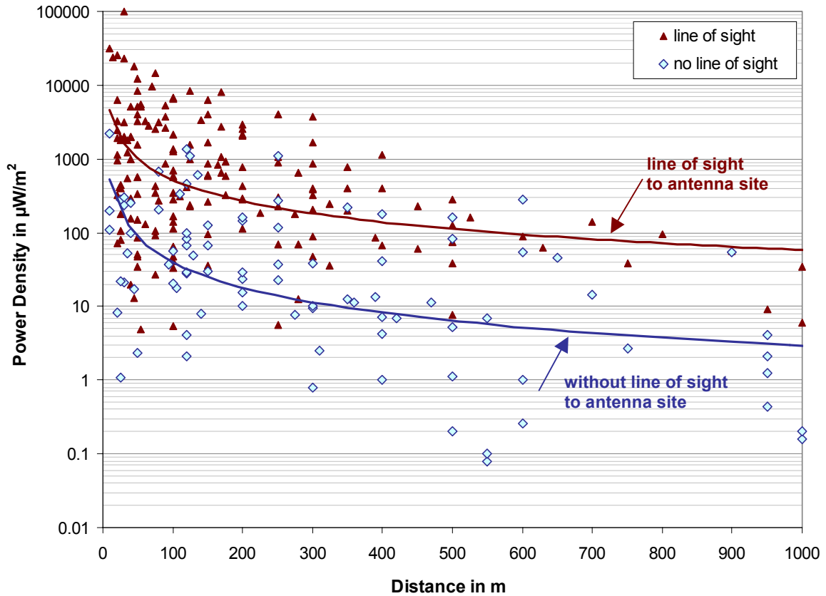
Figure 3: GSM cellular tower base station power density levels – line of sight and distance
